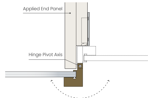
Cabinet with an Additional End Panel Maximum opening angle: 180°
