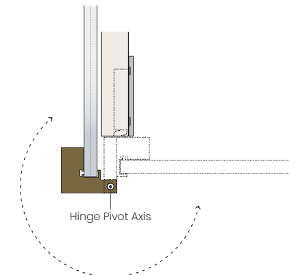
Cabinet without an Additional End Panel Maximum opening angle: 270°
