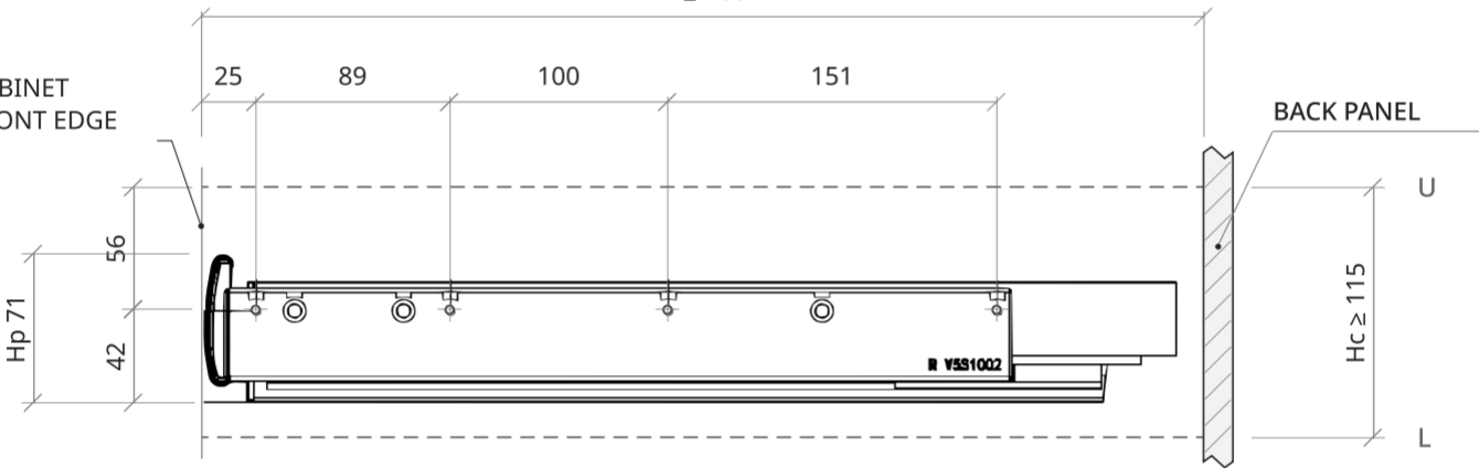
SIDE SECTION
