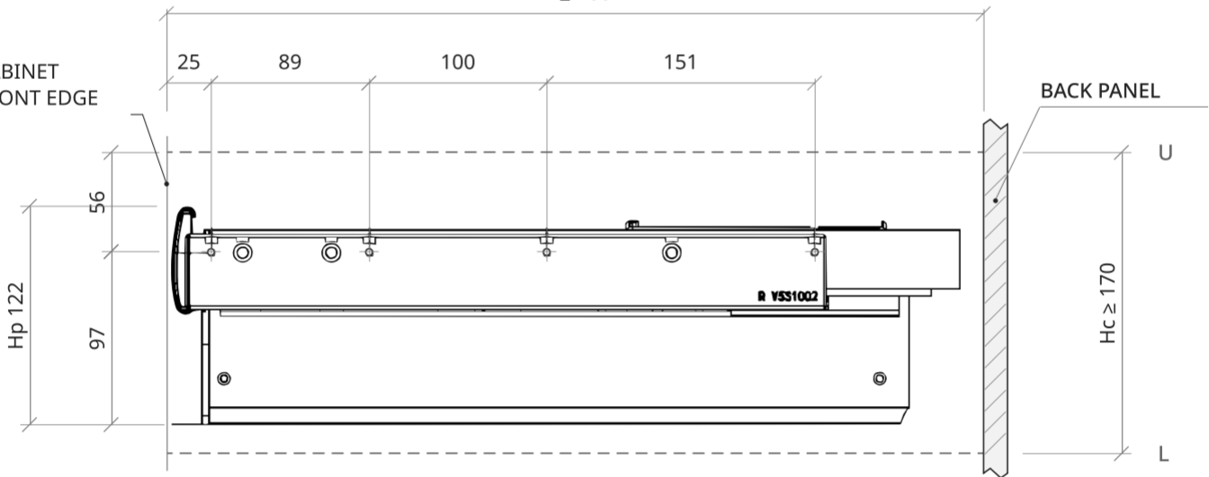
SIDE SECTION
